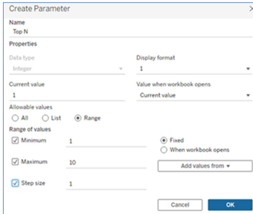
Figure 8.15: Create Parameter settings.
