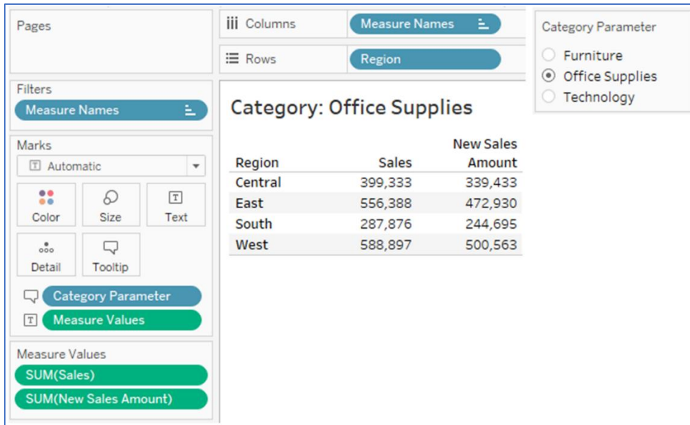
Figure 8.19: Region, Sales and New Sales with Parameter selection.
