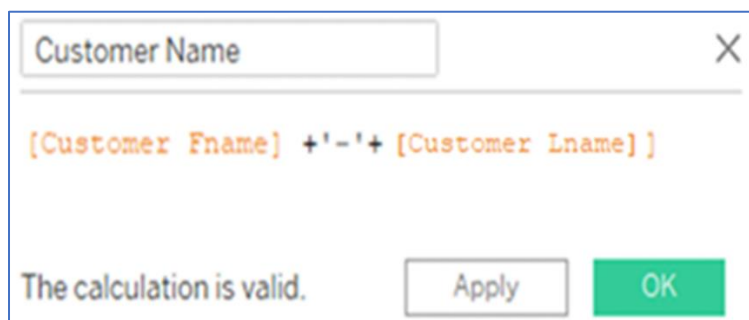
Figure 5.8: Calculation for creating Customer name.
