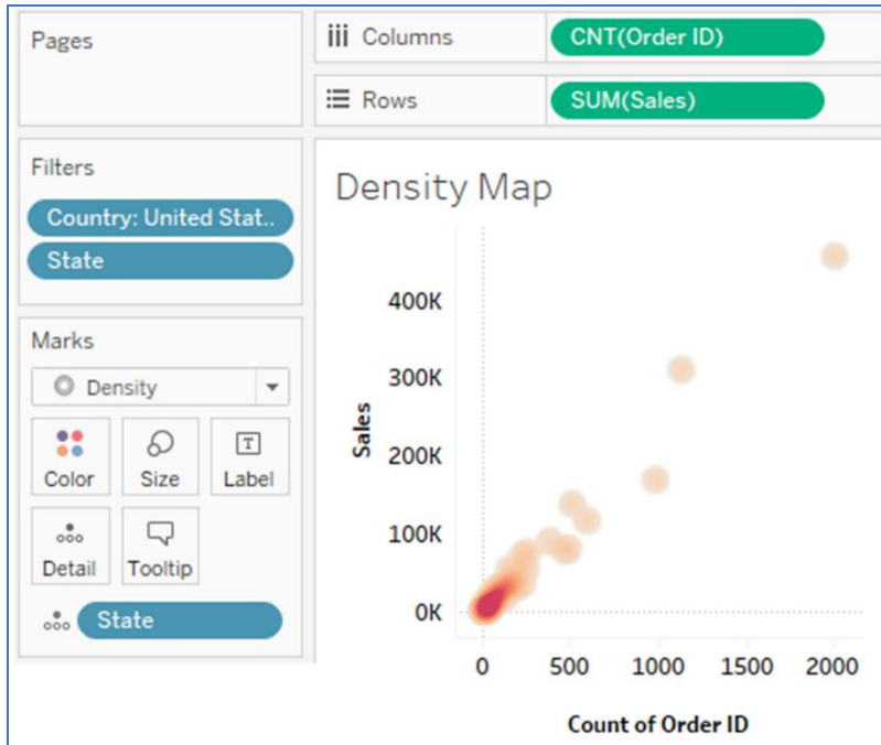
Figure 12.9: Density heat map.
