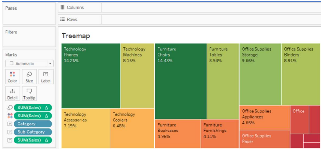
Figure 12.21: Treemap chart.
