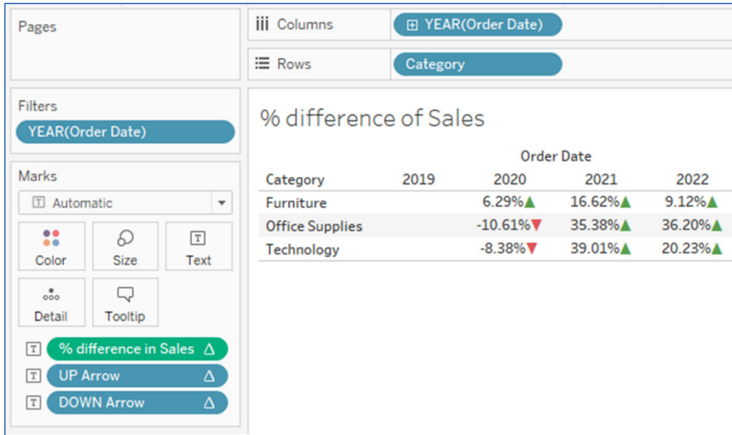
Figure 12.5: Text table with KPI arrows.
