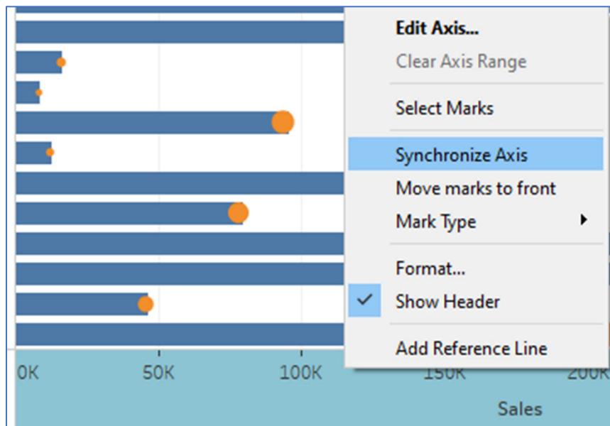
Figure 12.16: Synchronizing the axis.
