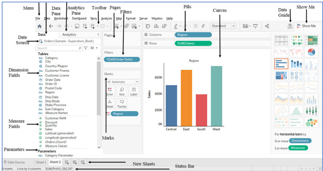
Figure 1.8: Tableau Desktop Workspace.
