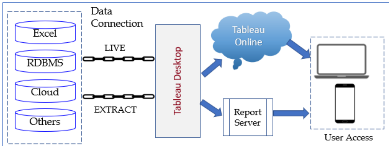
Figure 1.2: How Tableau Works.
